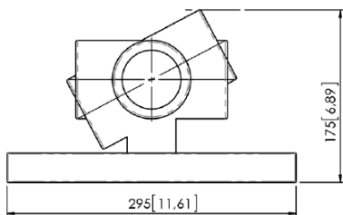
MAXIMUM CAMERA DIMENSIONS
