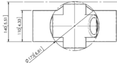
DIMENSION INCLUDING CONNECTORS
