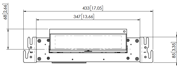
VIEW C
