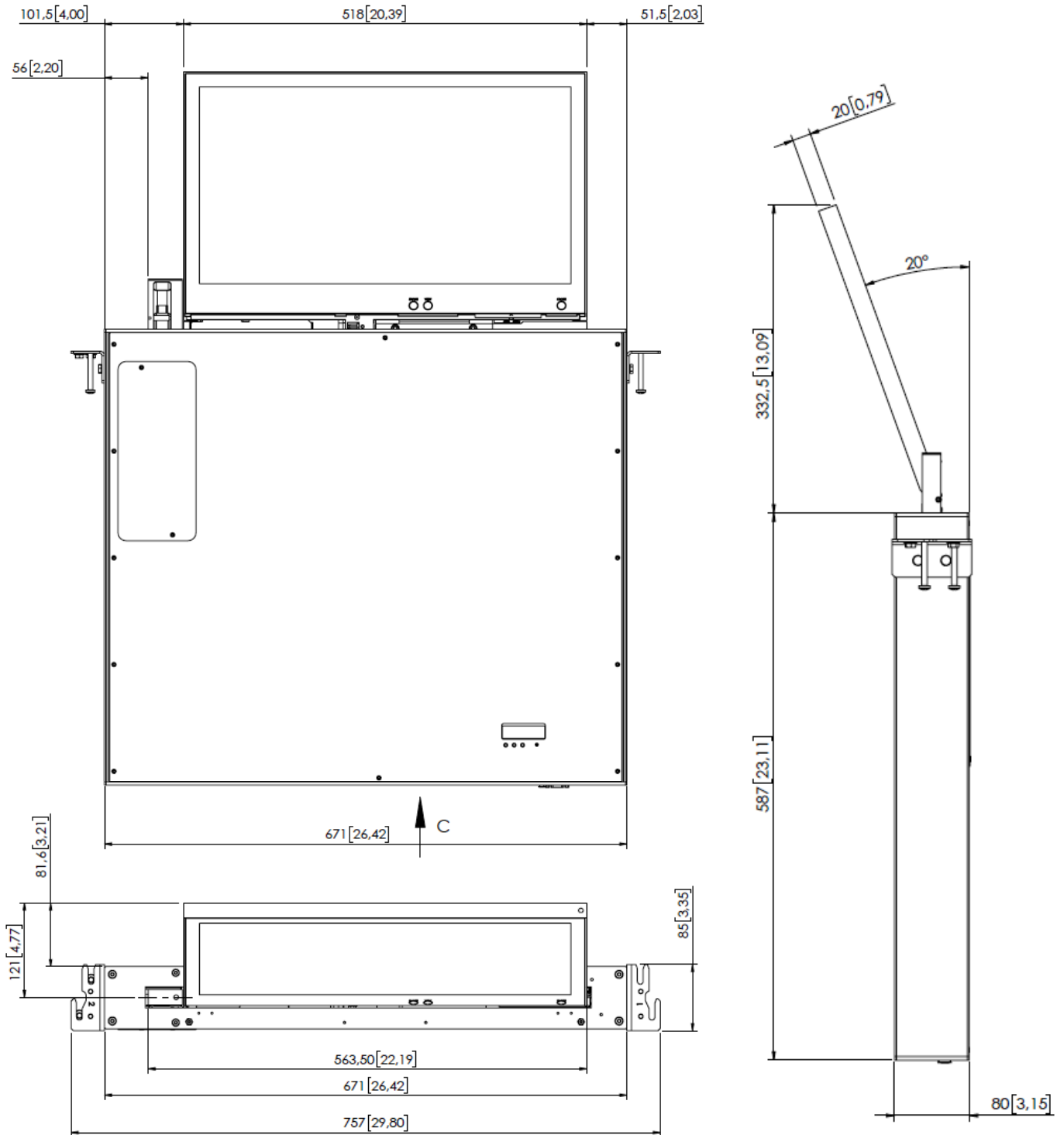
VIEW C
