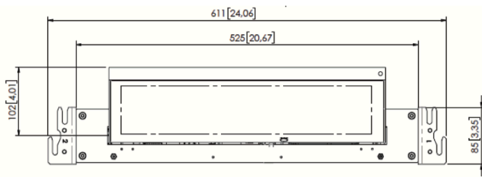
VIEW C
