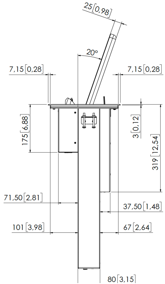
DX2KM 17 Maximum Keyboard/Mouse dimensions
