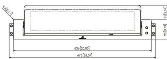
VIEW C
