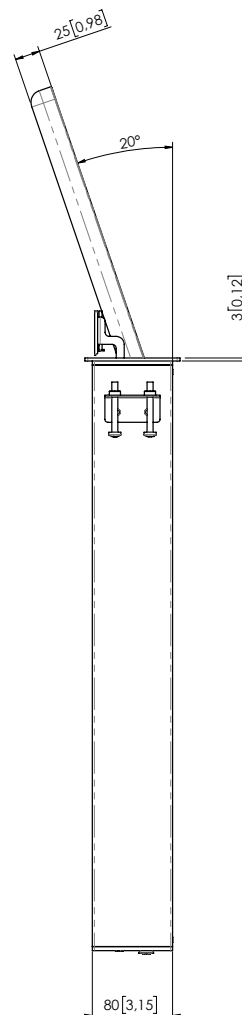
VIEW C
